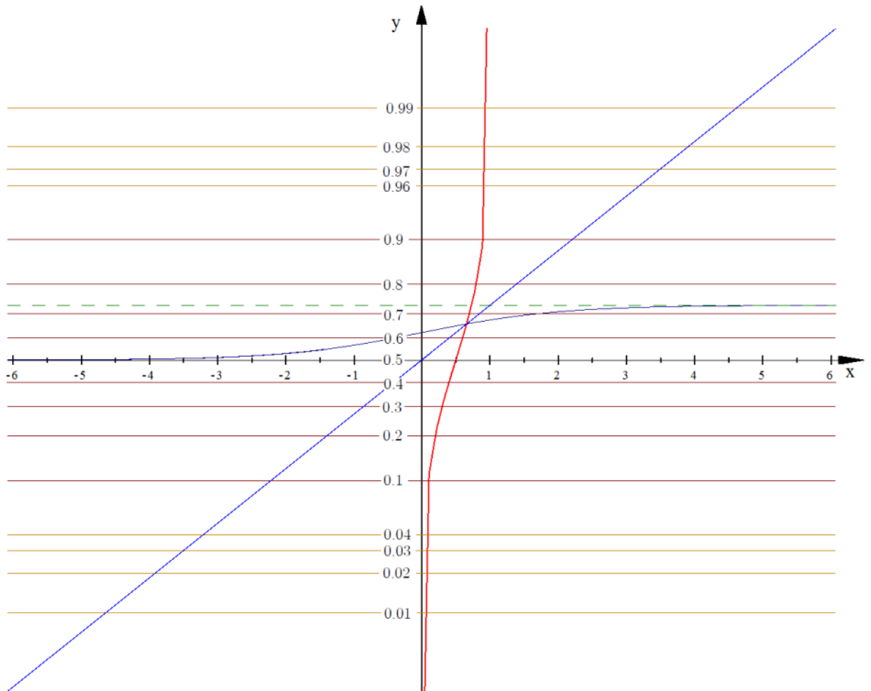
Figure 12: The function 1 - \frac{1}{1 + e^x} (blue) in the logit-x coordinate system
