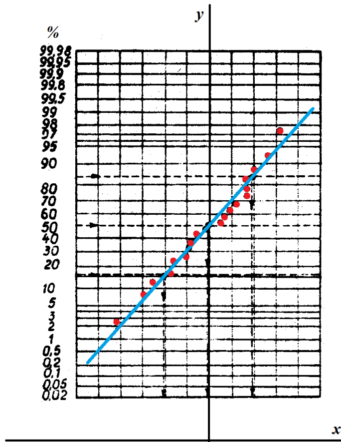
Figure 2: Gaussian coordinate system
